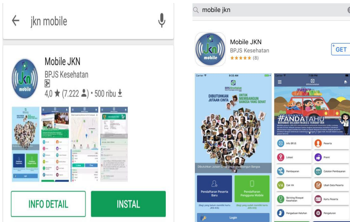
Android (Playstore)
